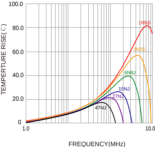
Temperature Rise VS. Frequency Characteristics:
